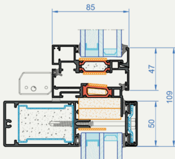
Automatic actuators version (example with facade AW50)
